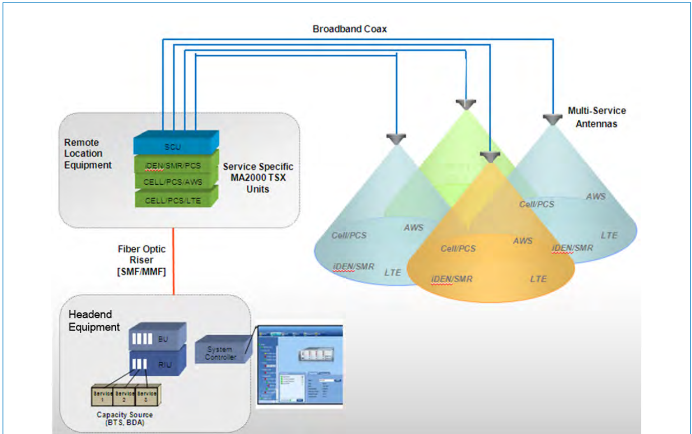
Example MA2000 TSX System Architecture | Figure 3
